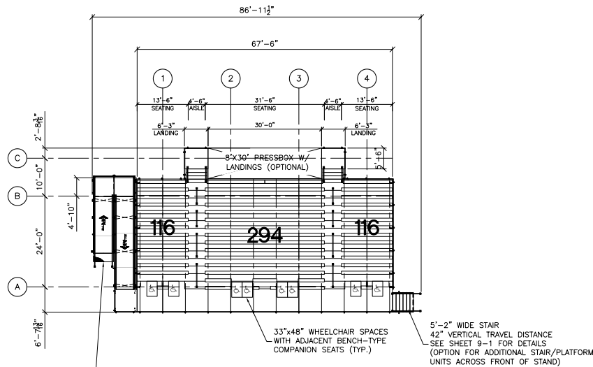
SEATING PLAN SCALE: 3/32" = 1'-0"
