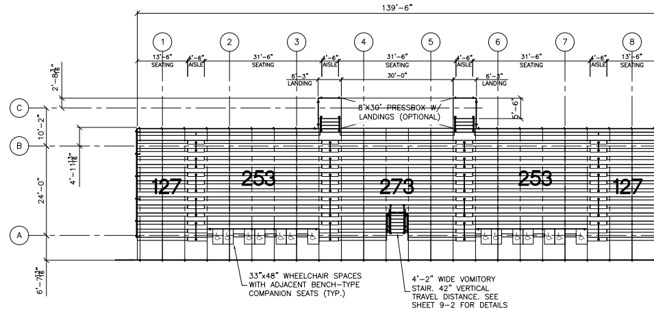
SEATING PLAN SCALE: 3/32" = 1'-0"
