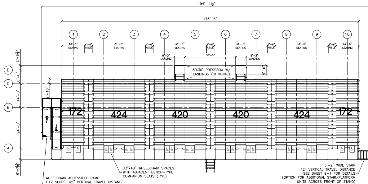
SEATING PLAN SCALE: 3/32" = 1'-0"
