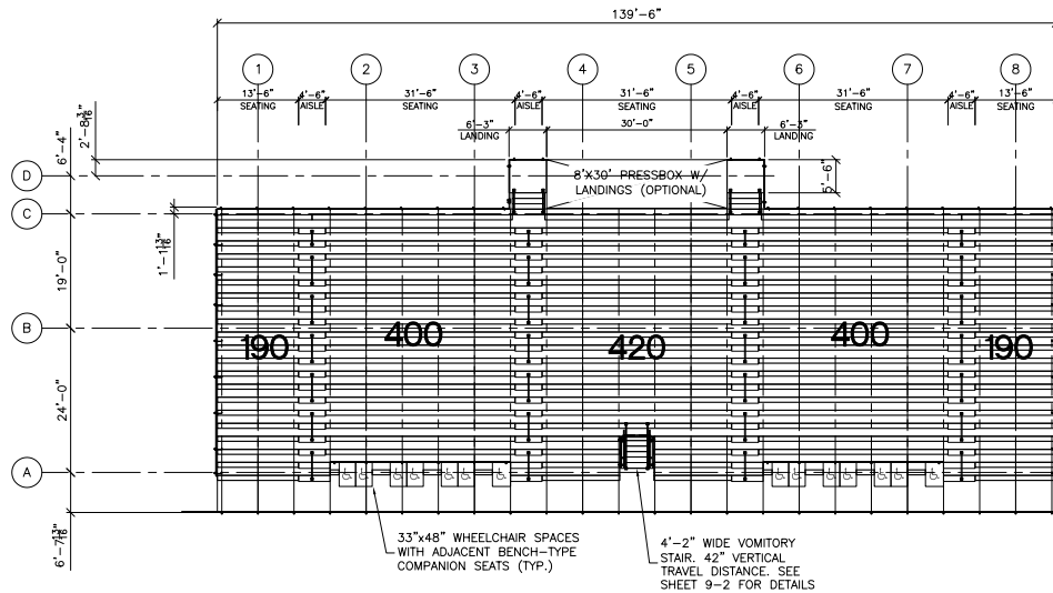
SEATING PLAN SCALE: 3/32" = 1'-0"
