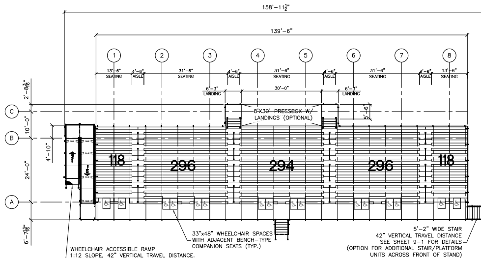
SEATING PLAN SCALE: 3/32" = 1'-0"
