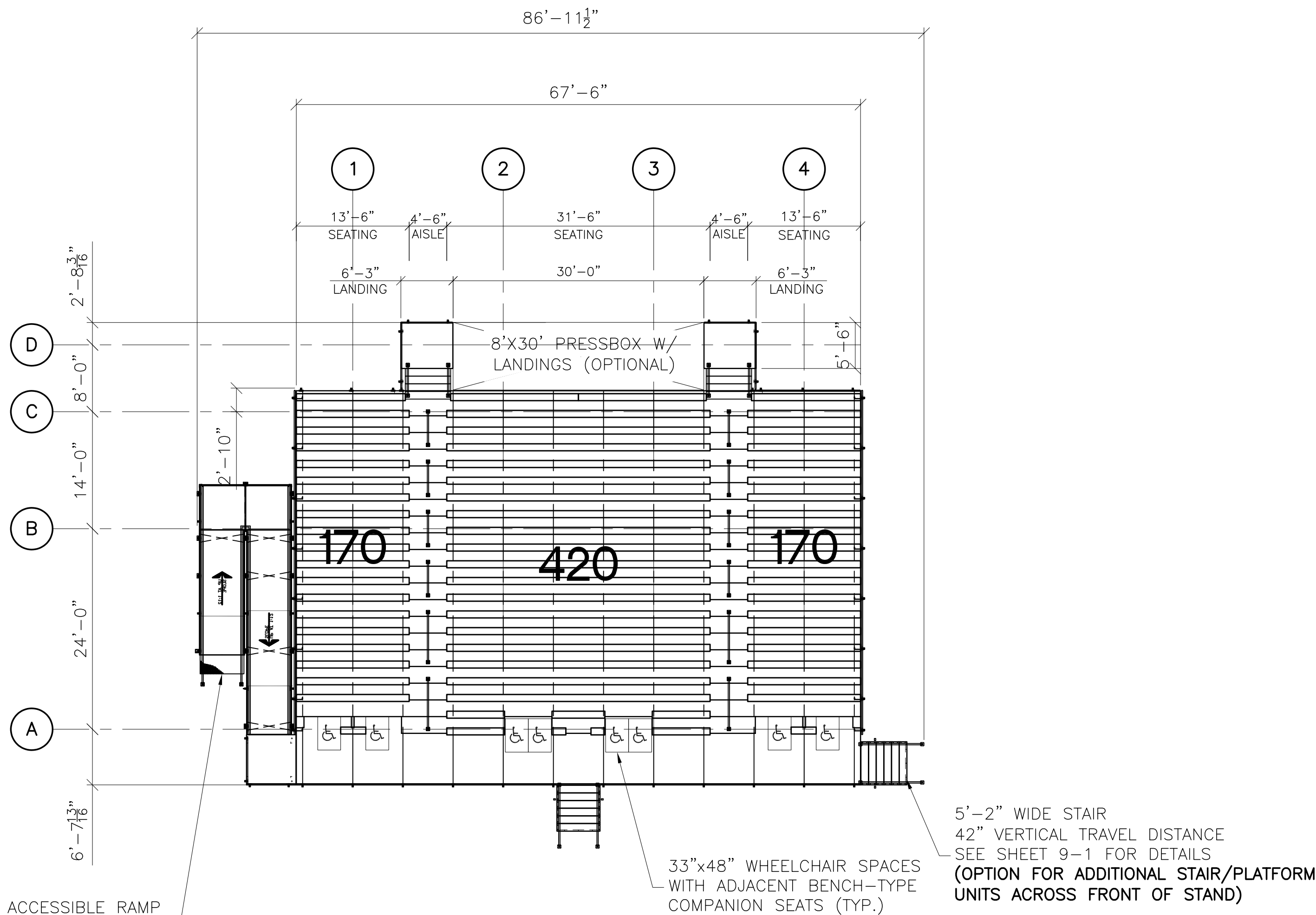
SEATING PLAN SCALE: 3/32" = 1'-0"
