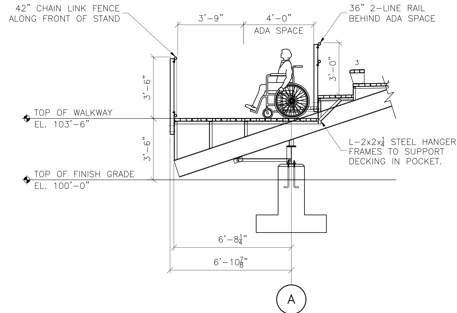
2 SECTION THRU BLEACHER AT ADA POCKET
