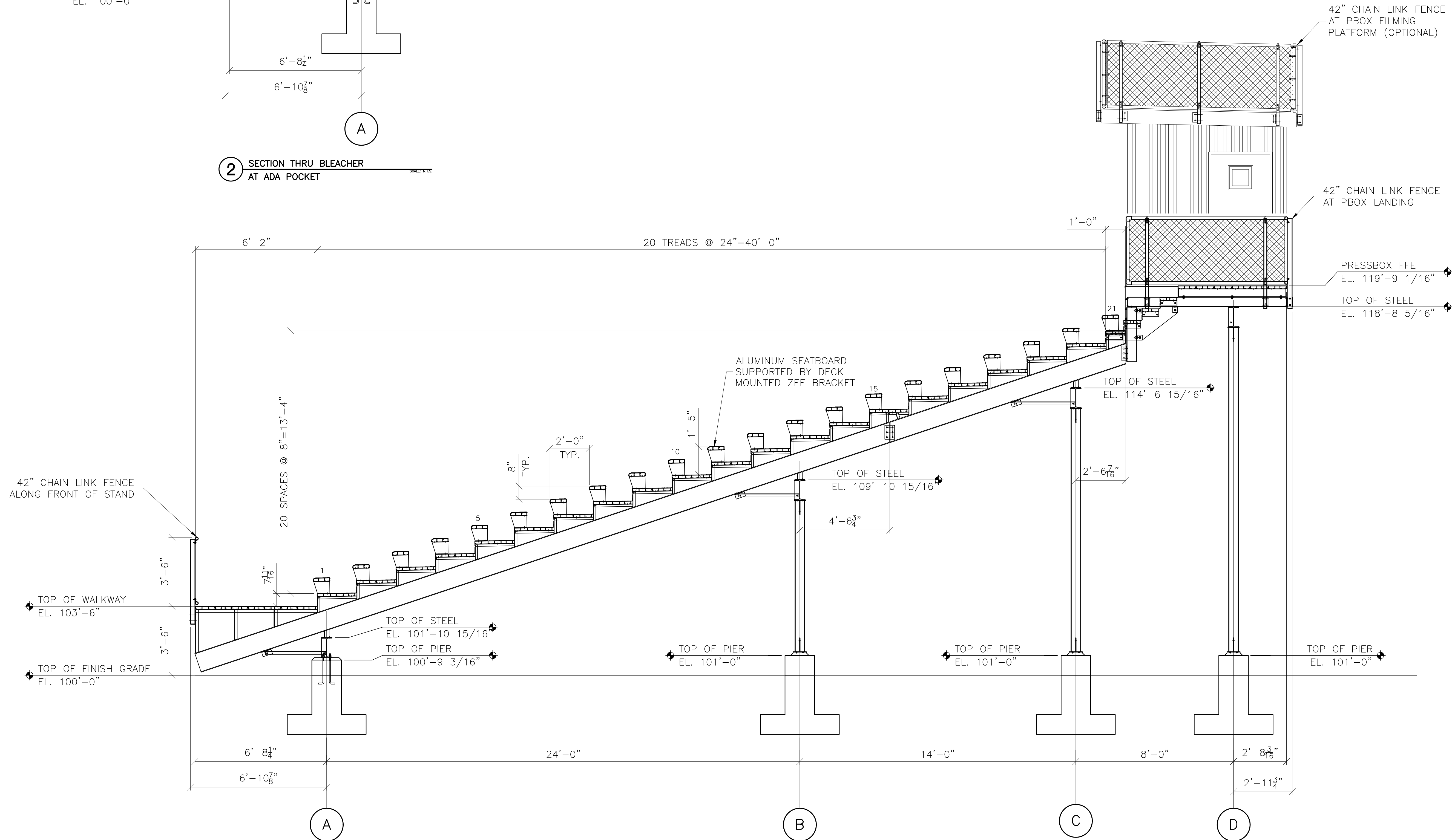
1 SECTION THRU BLEACHER AT SEATING
