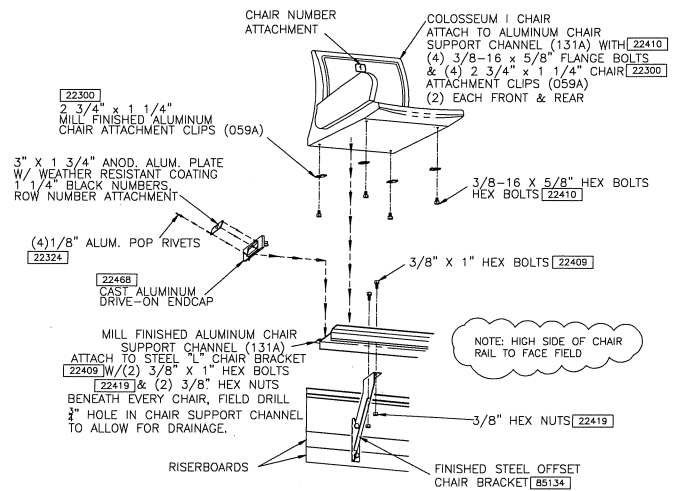
COLOSSEUM I CHAIR INSTALLATION
