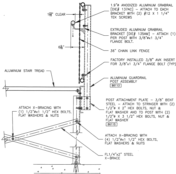
SECTION THRU STAIR STRINGER
