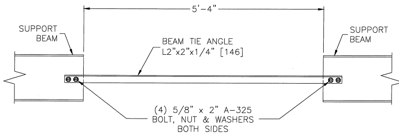
Tie Angle to Support Beam Connection
