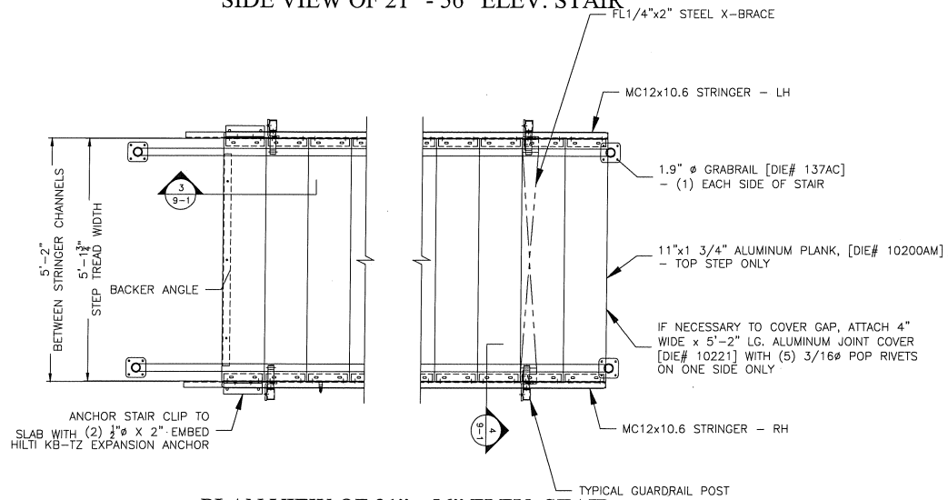
PLAN VIEW OF 21" - 56" ELEV. STAIR
