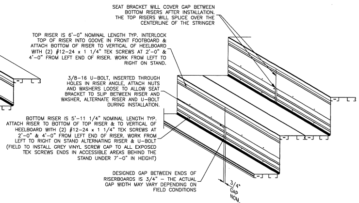
Figure 2 Riser to Decking Connection
