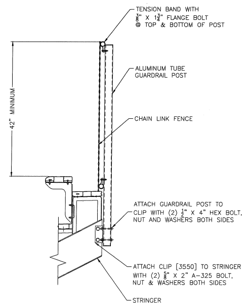
TYPICAL GUARDRAIL CONNECTION AT REAR OF STAND
