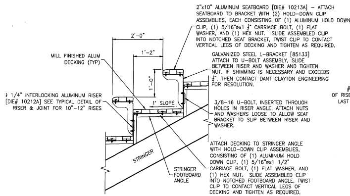
Figure 1 Seat Bracket to Stringer - L Bracket
