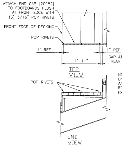
END CAP TO FOOTBOARD
