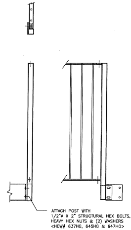
LEVEL PANELS TO END POST AT REAR
