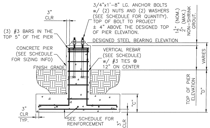
Typical Column to Pier Connection
