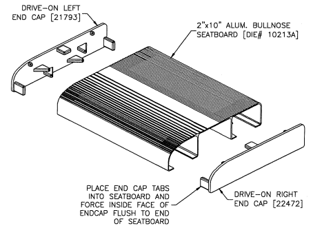
END CAP FOR SEATBOARD
