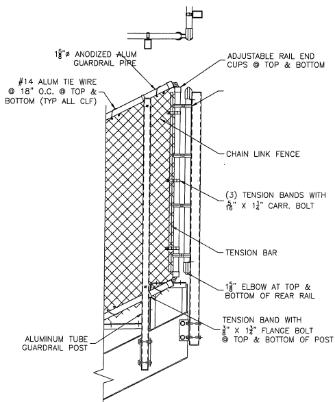
REAR CORNER GUARDRAIL DETAIL
