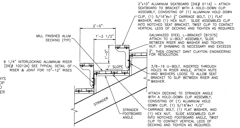
TYPICAL FOOTBOARD DECKING TO STRINGER CONNECTIONS
