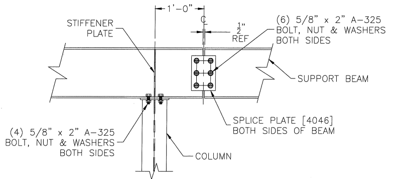
Typical Splice Connection Support Beam over Column
