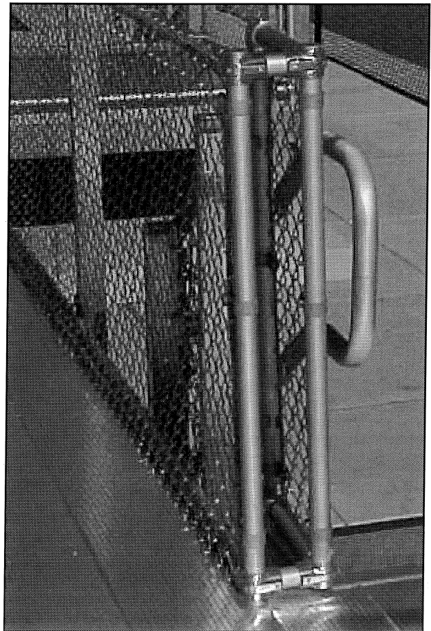
INSTALLED FILLER PANEL (USED IF GREATER THAN 4")
