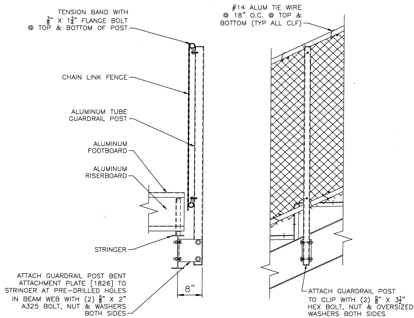
TYPICAL GUARDRAIL CONNECTION AT SIDE OF STAND
