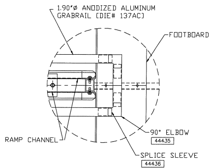
CONNECTION OF GRABRAIL AT INSIDE OF LANDING
