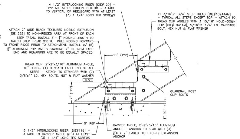
SECTION THRU BOTTOM STEPS
