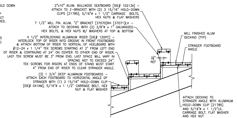
Figure 2 Seat Bracket to Stringer - Z Bracket
