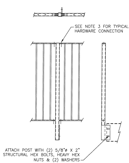
LEVEL PANELS & INT POST AT FRONT
