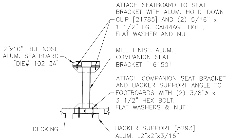
Figure 1 Companion Seat to Decking
