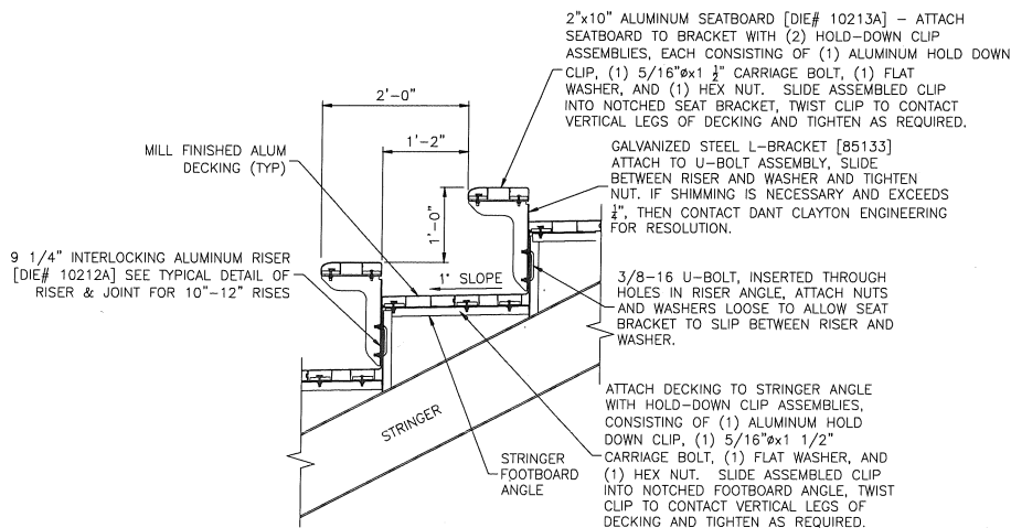
SEAT BOARD TO SEAT BRACKET
