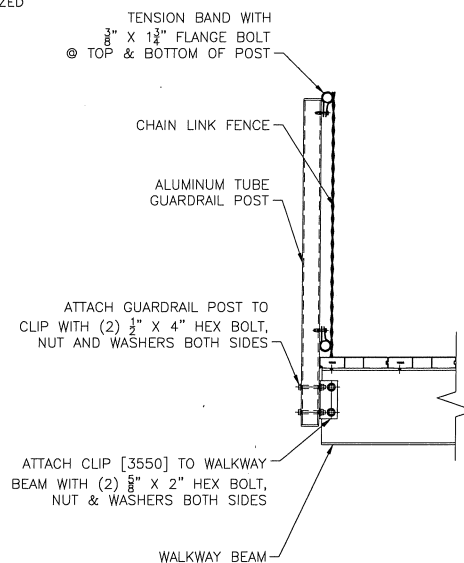
TYPICAL GUARDRAIL CONNECTION AT FRONT OF STAND
