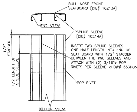
SPLICING OF SEATBOARD CONNECTION
