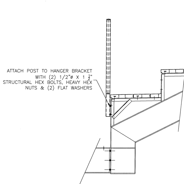
CONNECTION OF LEVEL PANEL & END POST AT REAR OF HC AREA
