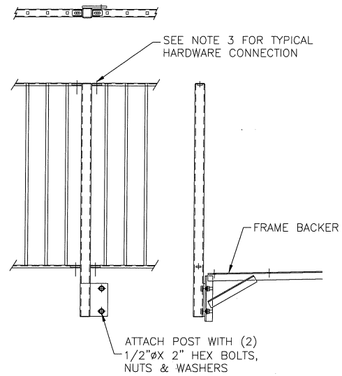
CONNECTION OF LEVEL PANEL & INT. POST AT REAR OF HC AREA
