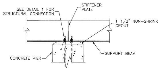
Support Beam to Pier Connection
