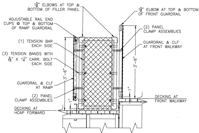
FILLER PANEL AT CROSS-AISLE & HCAP SEATING SECTION
