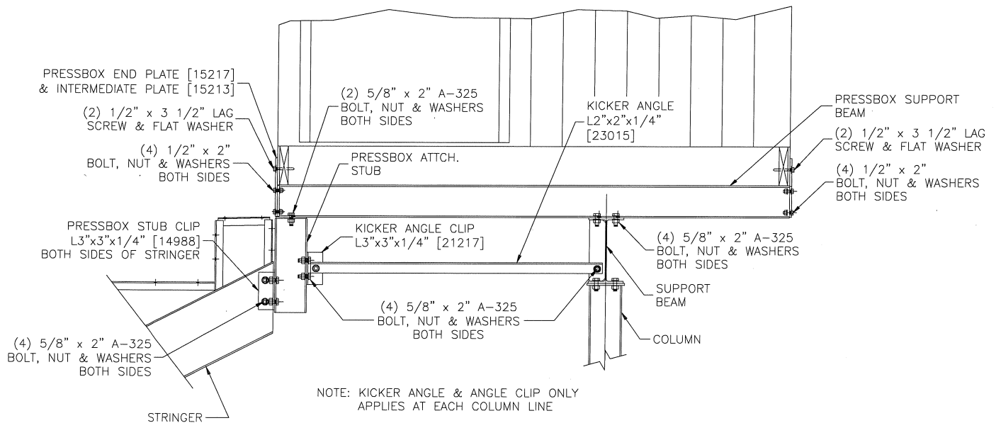
Press Box Beam To Press Box Stub Connection / Press Box to Press Box Beam Connection
