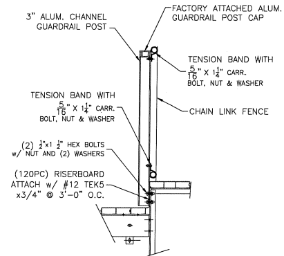
REAR GUARDRAIL POST AT HCAP AREA
