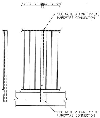
PANEL & POST AT FRONT
