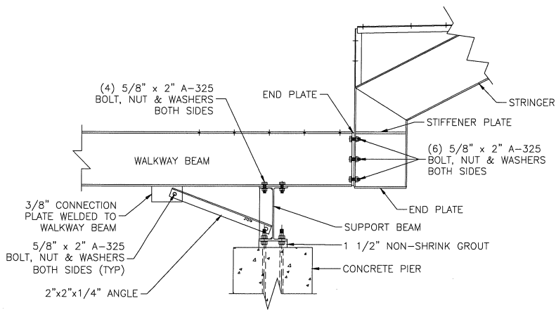
Typical Walkway Connection Beam to Pier 12/24 Stringer
