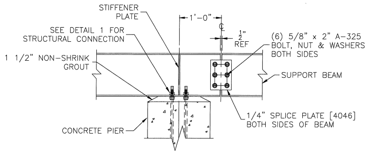
Typical Splice Connection Support Beam over Pier
