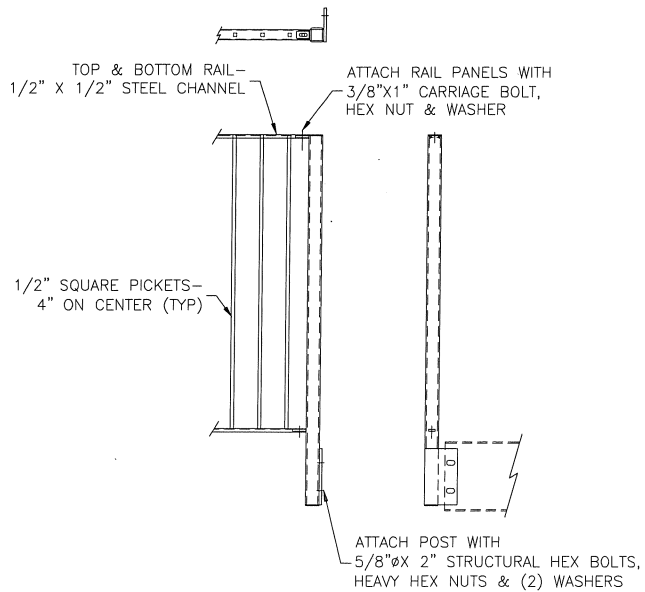
LEVEL PANEL & END POST AT FRONT/ REAR
