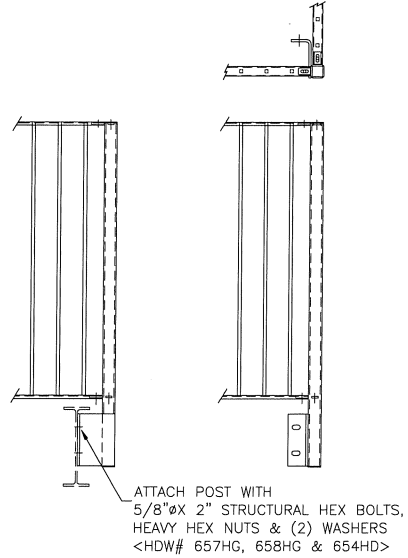
LEVEL PANELS & CORNER AT FRONT/ SIDES
