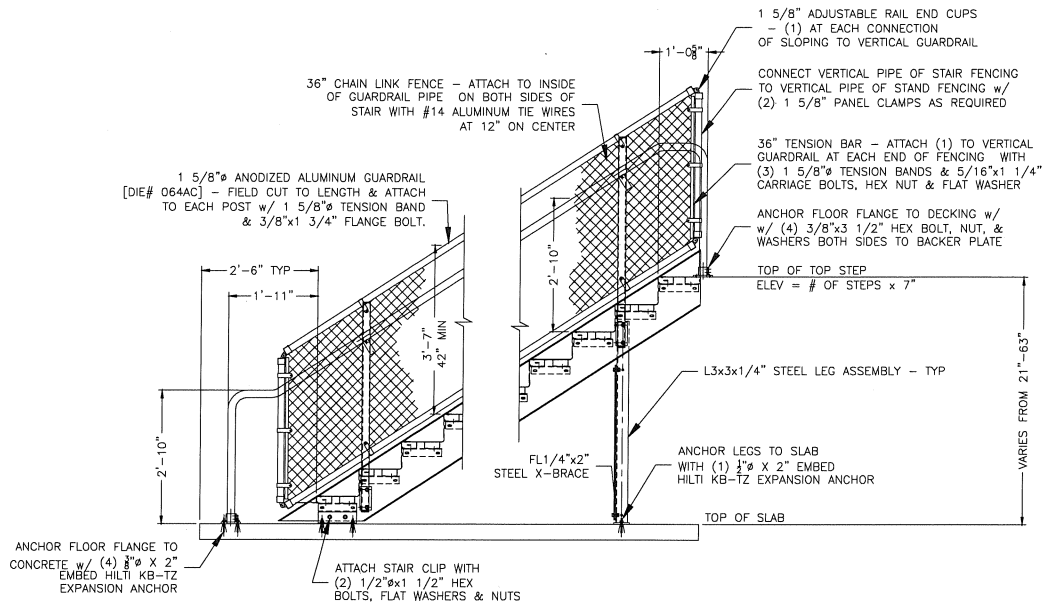
SIDE VIEW OF 21" - 56" ELEV. STAIR
