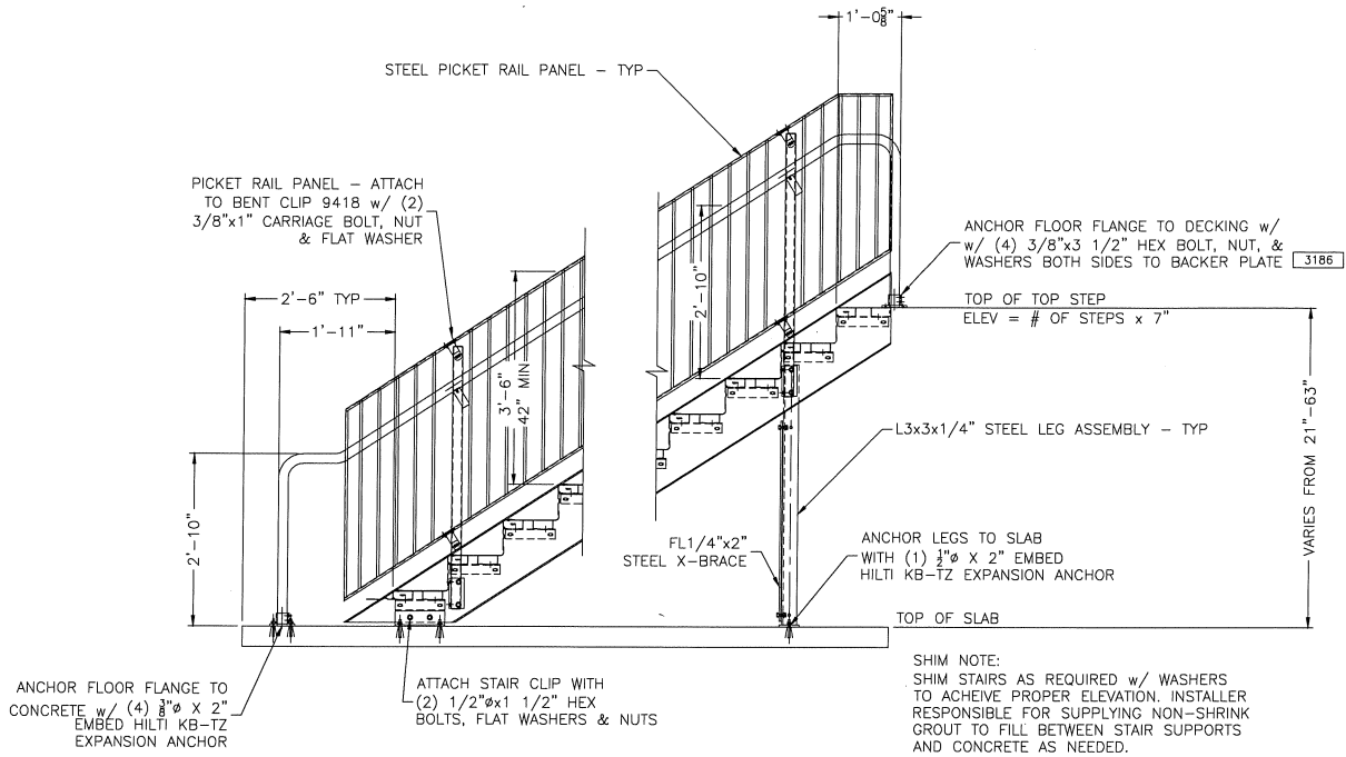
SIDE VIEW OF 21'-56" ELEVATED STAIRS
