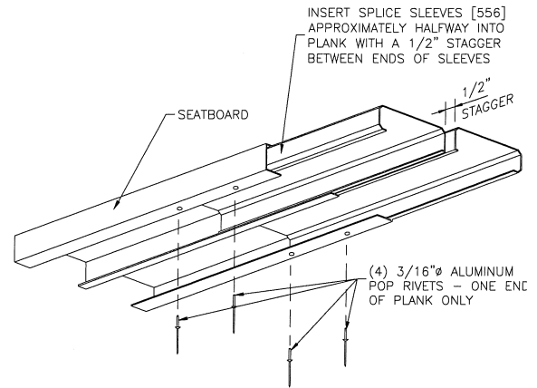
SPLICING OF SEATBOARD BOTTOM VIEW
