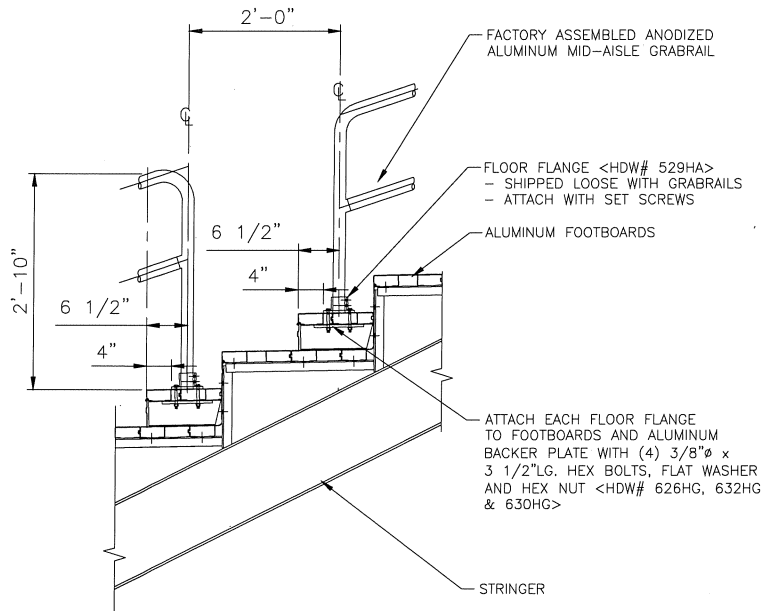
Figure 1 NFPA Installation of Intermediate Step (Side View)
