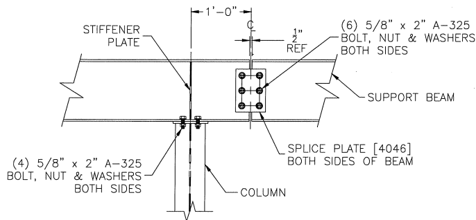
Support Beam to WF Column Connection
