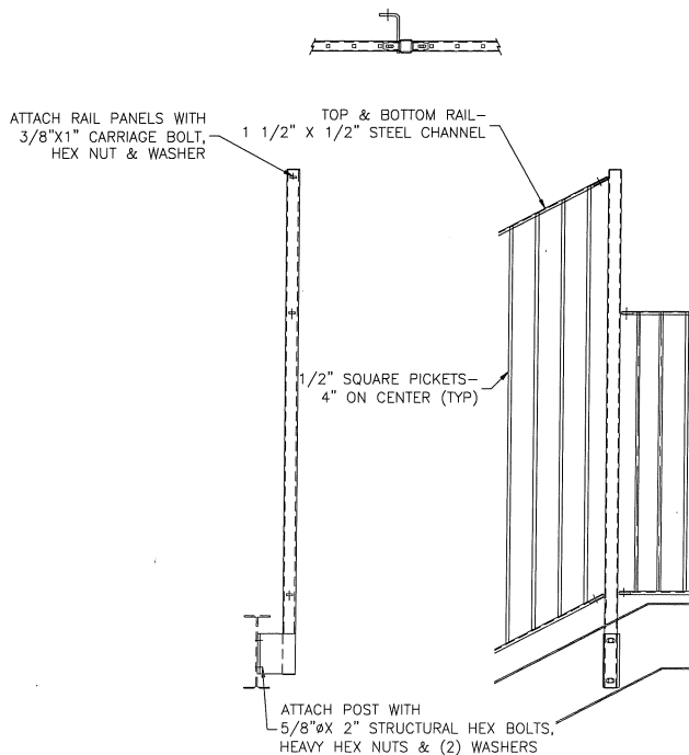
CONNECTION OF LEVEL AND SLOPED PANELS TO INT. POST AT SIDE
