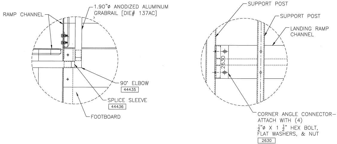
CONNECTION OF GRABRAIL AT CORNER OF LANDING
