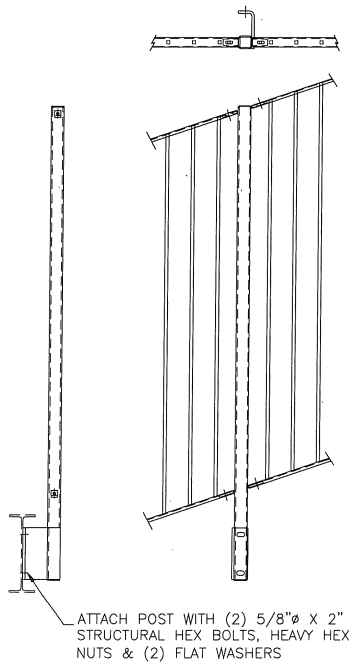
SLOPED PANEL & INT. POST AT SIDES
