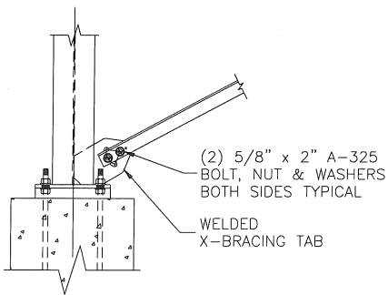
Cross Bracing to WF Column Connection
