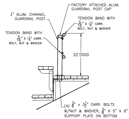
2-LINE RAIL AT CROSS AISLE
