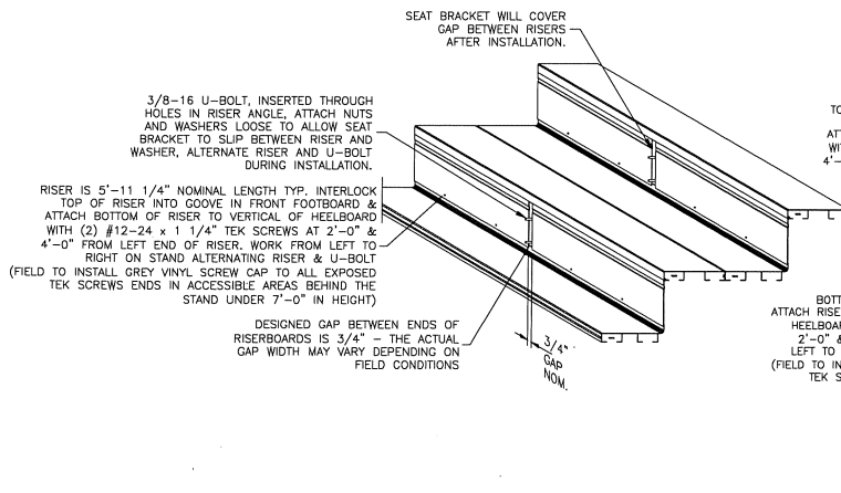
Figure 1 Riser Connection
