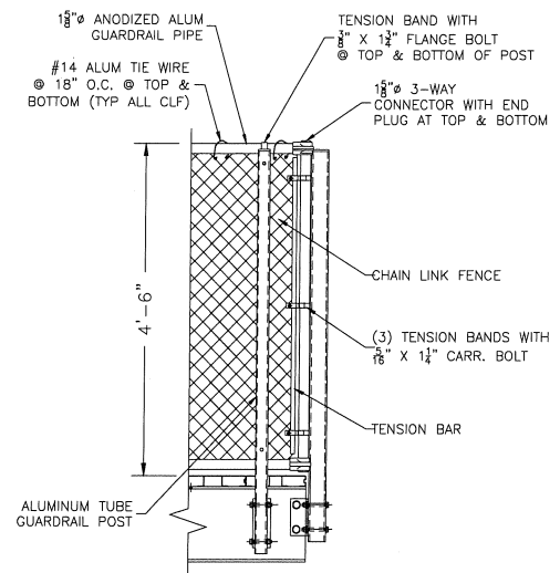
2 RAIL CLF CONNECTION AT REAR OF STAND
