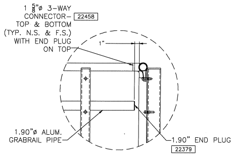
TERMINATION OF GRABRAIL AT
