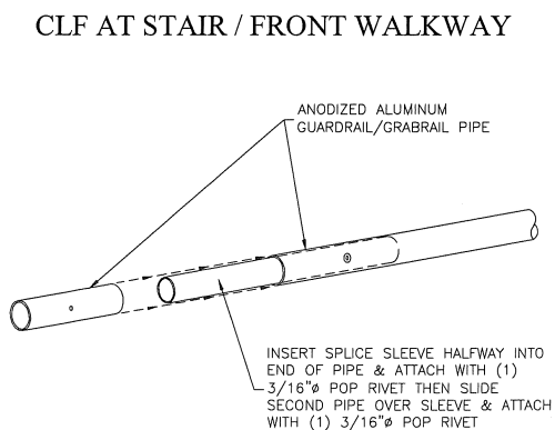
TYP. GUARD/HAND RAIL SPLICE DETAIL
