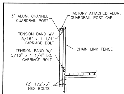
FRONT GUARDRAIL POST AT HCAP AREAS
