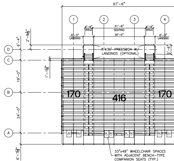
SEATING PLAN SCALE: 3/32" = 1'-0"
