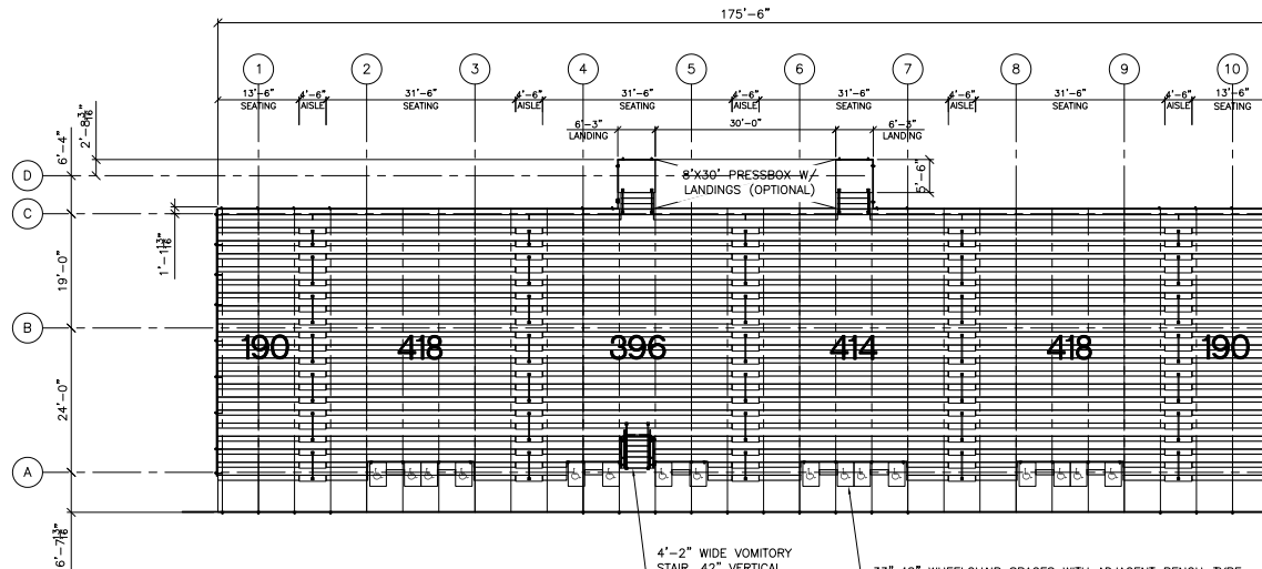
SEATING PLAN SCALE: 3/32" = 1'-0"
