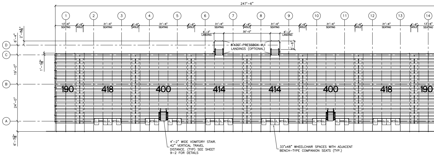
SEATING PLAN SCALE: 3/32" = 1'-0"
