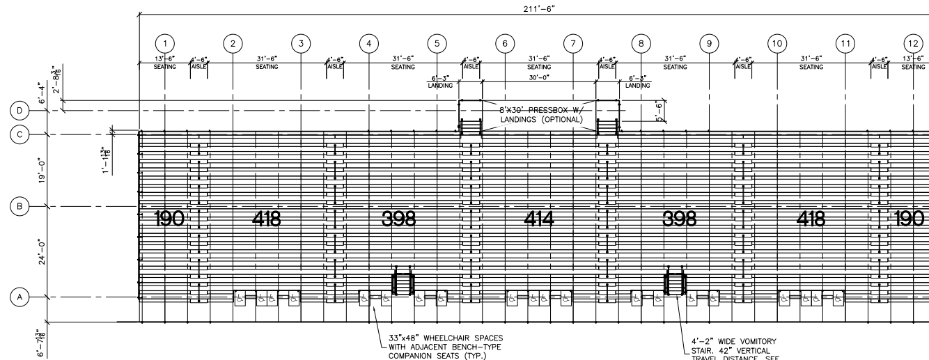
SEATING PLAN SCALE: 3/32" = 1'-0"
